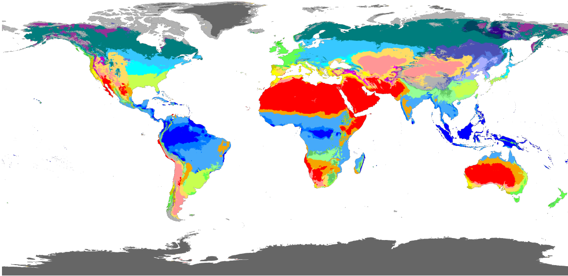
Figura 9: Köppen–Geiger climate classification (1980–2016). Source: Wikimedia Commons (see figures/koppen_climate.png.license.txt for attribution).
